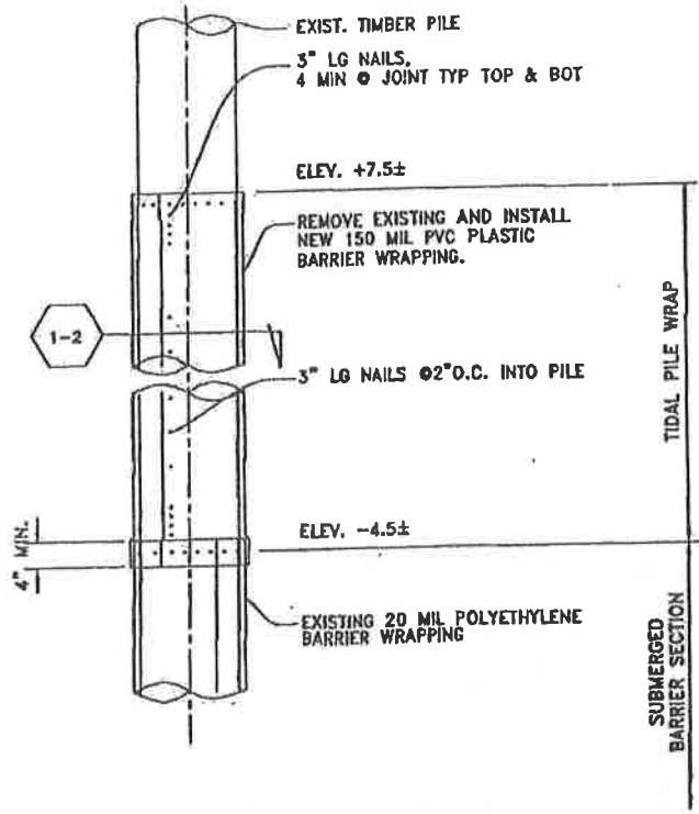
1-1 TIDAL WRAP ELEVATION - RECONSTRUCTION OF EXISTING FENDER PILE WRAPPING NEW FENDER PILE WRAPPING, SIMILAR SCALE: NTS
