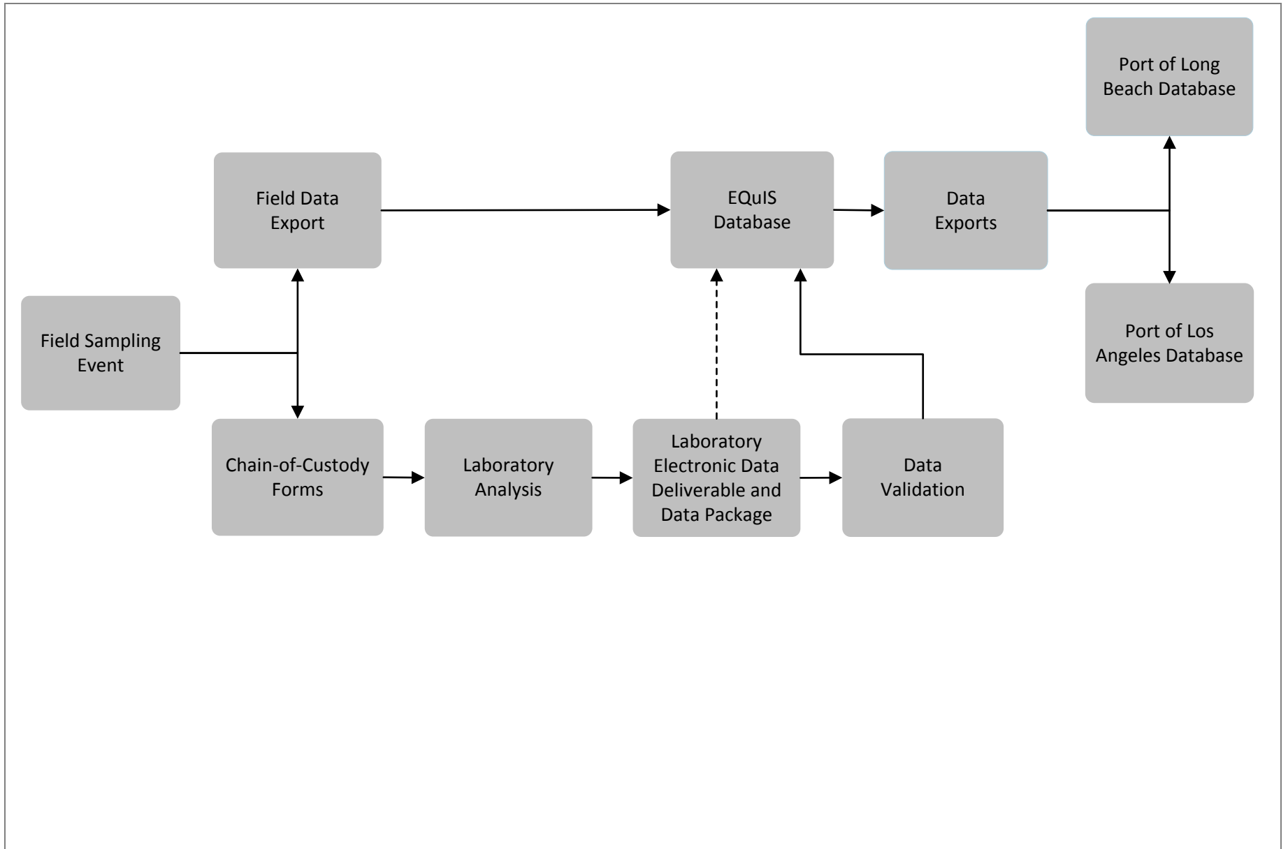
Figure 8 Data Flow Diagram
