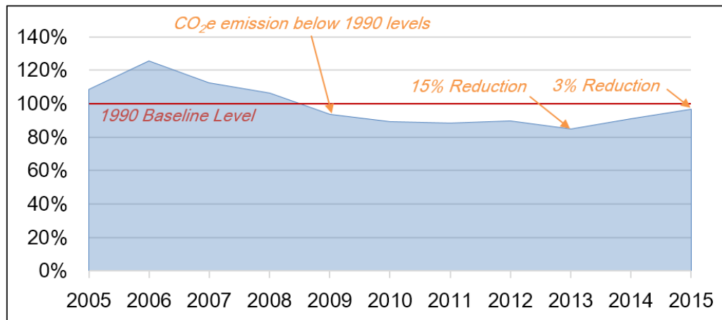
Figure 3: GHG Emissions 2005–2015
