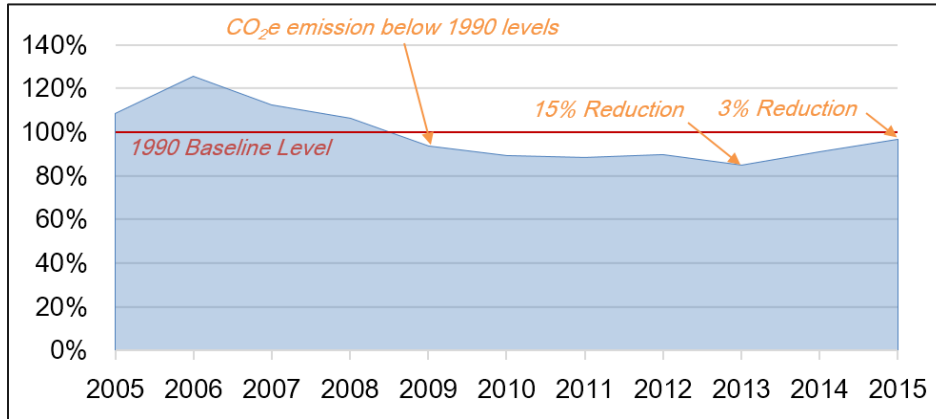
Figure 4.7-1: GHG Emissions 2005–2015
