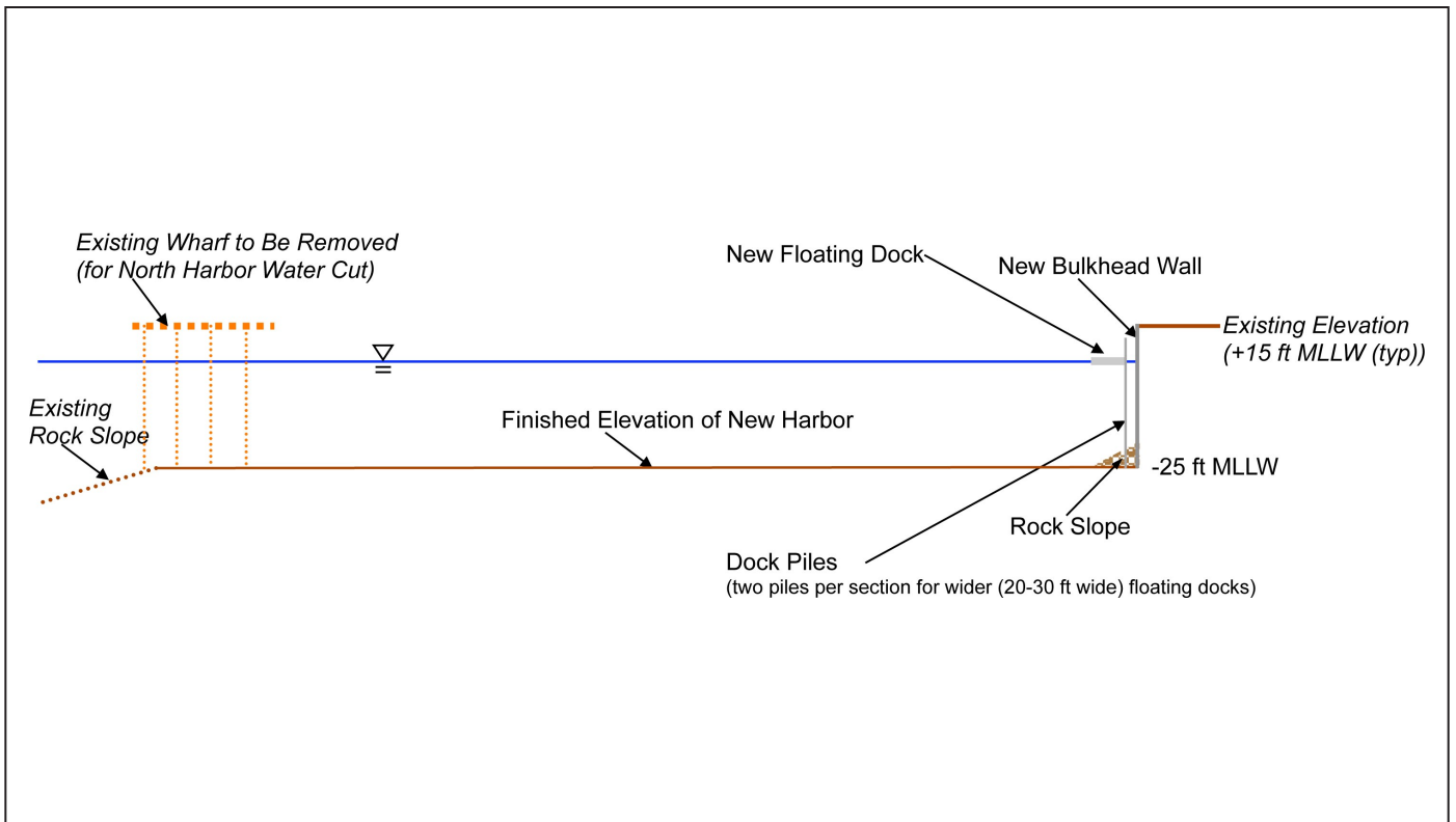
1b. Conceptual Representative Cross Section of New Harbor Cuts Alternate Perimeter—Rock Slope along Perimeter
