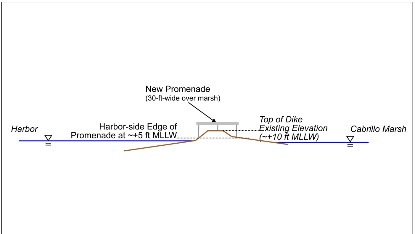
7. Conceptual Representative Cross Section along Salinas de San Pedro Salt Marsh
