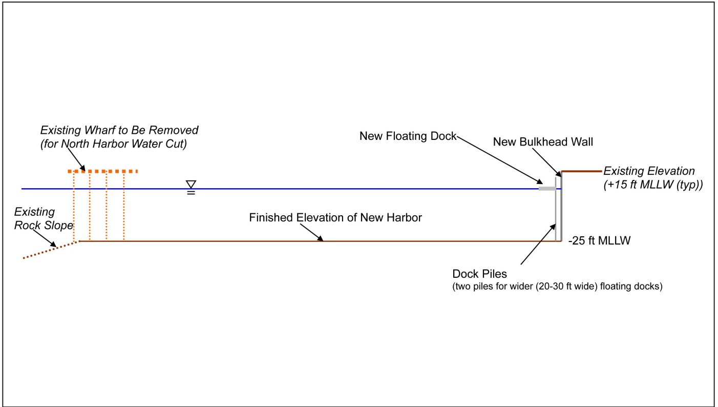
1a. Conceptual Representative Cross Section of New Harbor Cuts
