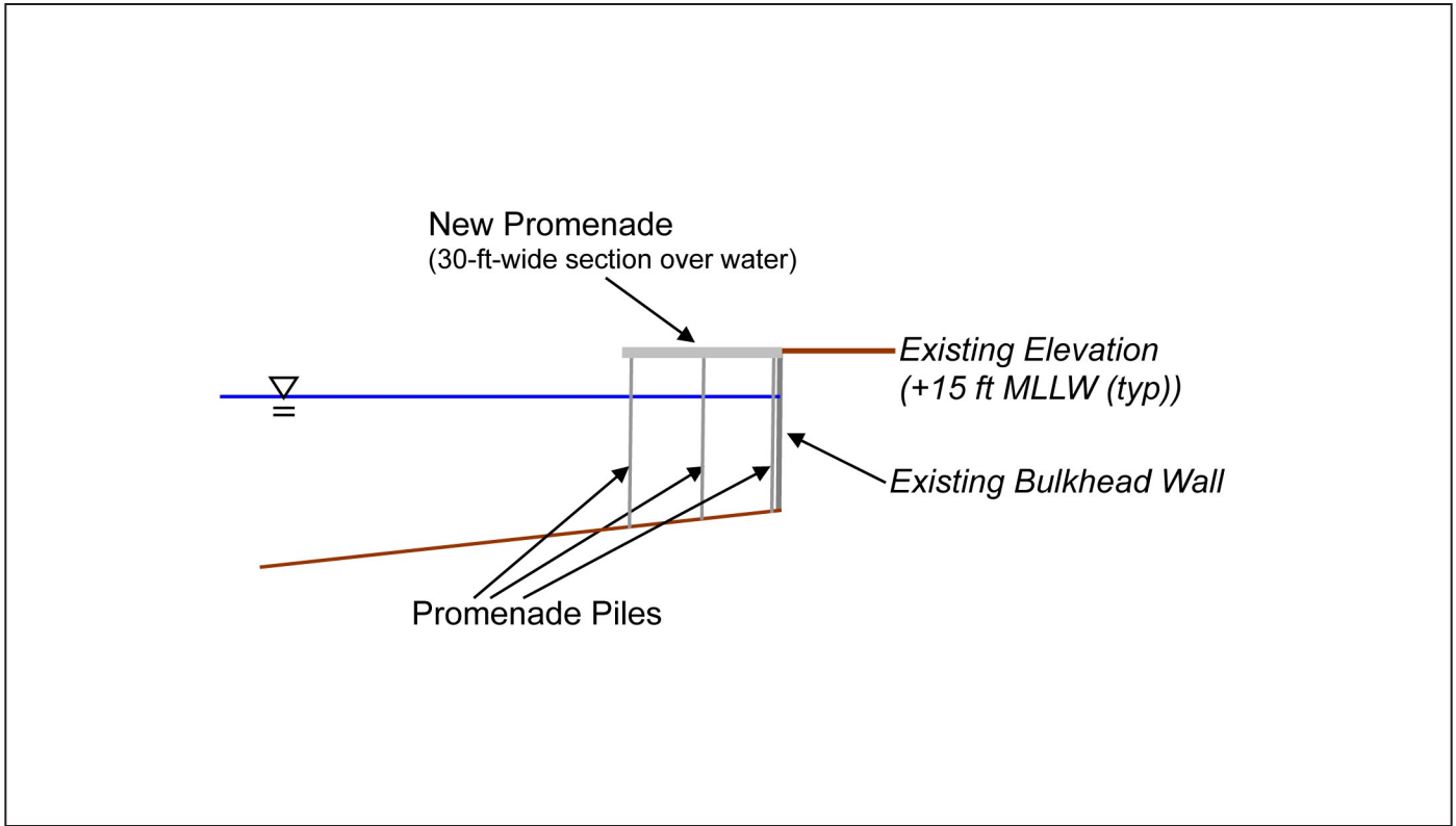
2. Conceptual Representative Cross Section along POC Promenade 30-ft Wide Waterside Promenade Section
