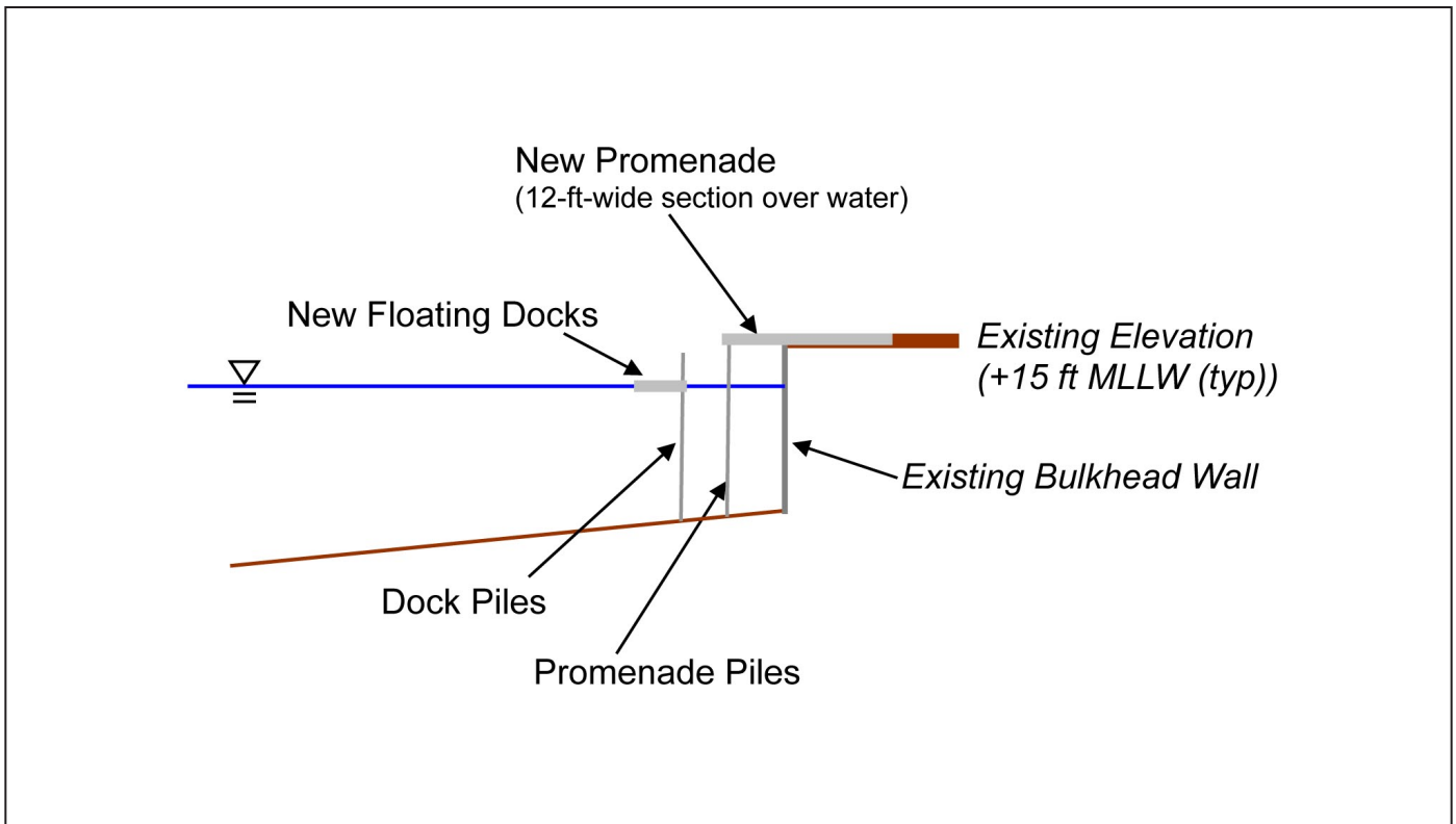
3. Conceptual Representative Cross Section along POC Promenade 12-ft Wide Waterside Promenade Section
