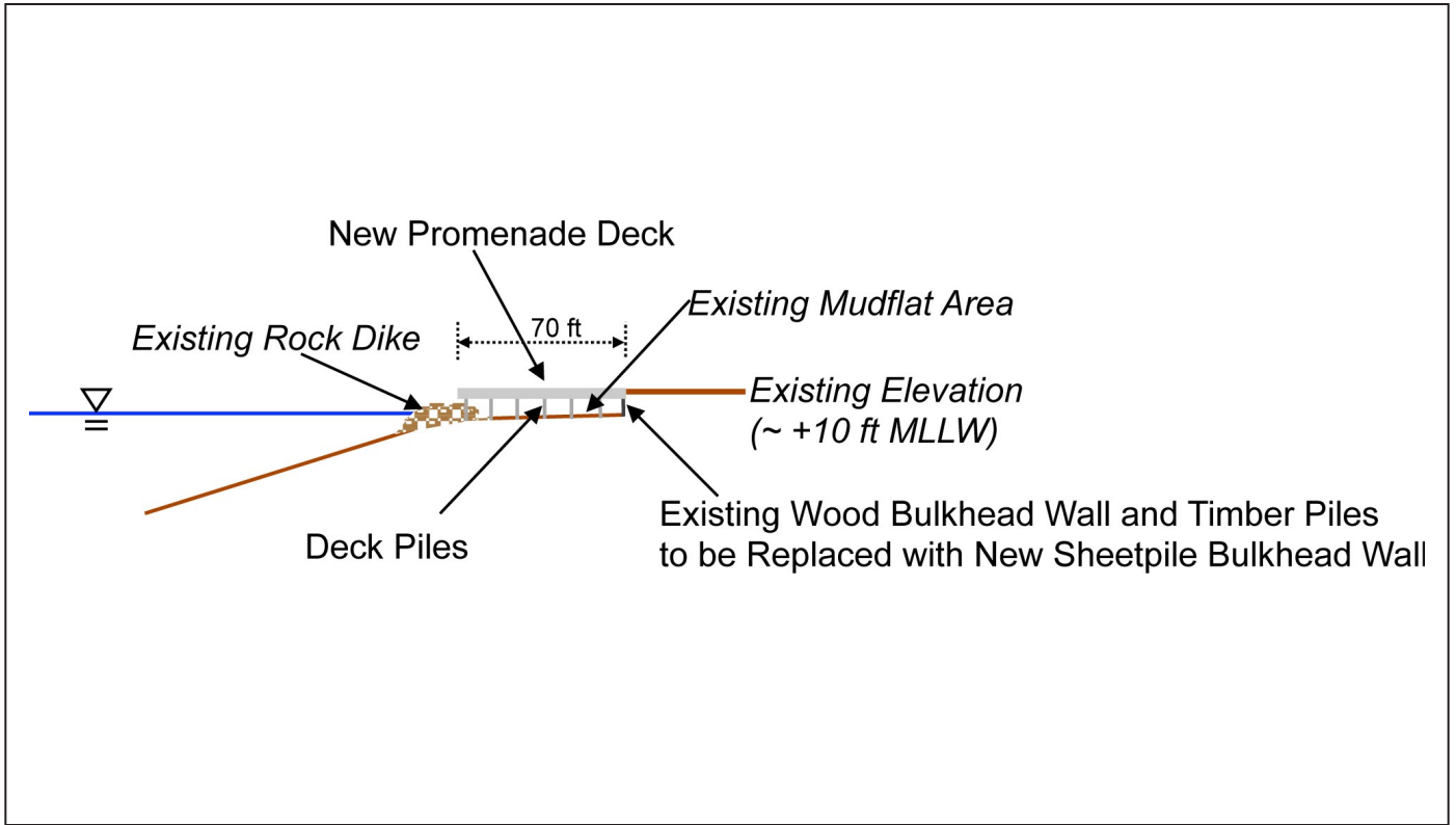
6. Conceptual Cross Section at Berth 78 Mudflat
