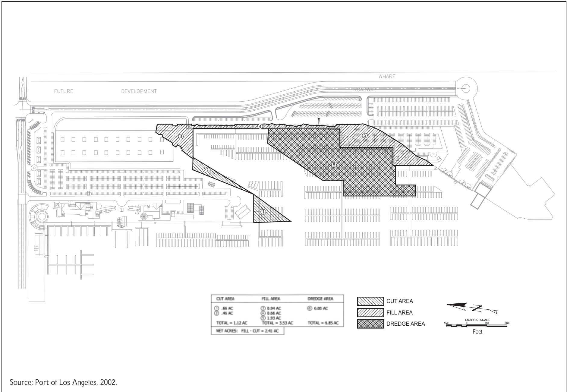
Figure 2-8 Proposed Cut, Fill, and Dredge Areas
