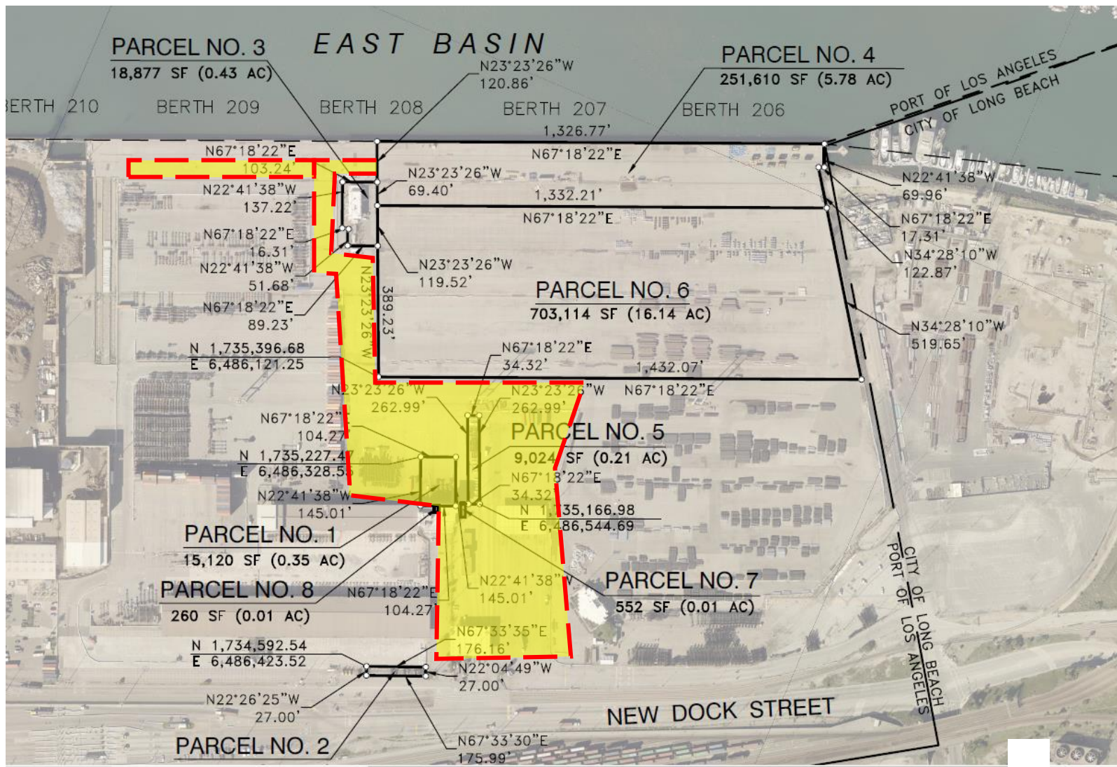
Secondary Premises/Flex Area
