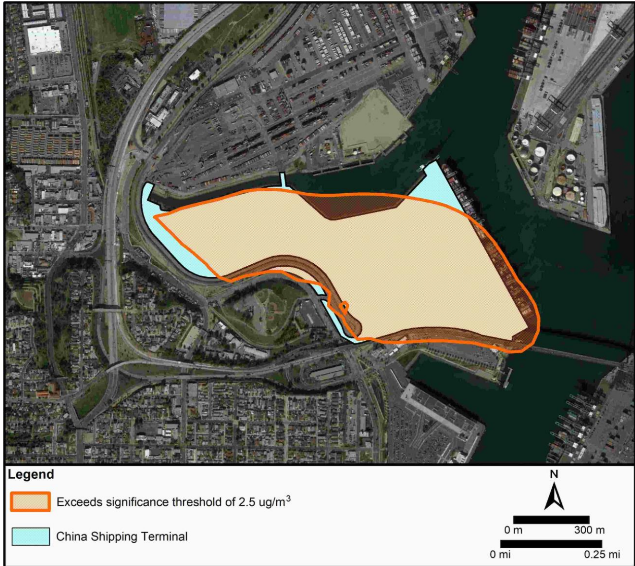
Figure B2-29. Area of Threshold Exceedance for the FEIR Mitigated Scenario; 2030 24-Hour PM 10 Concentration Increments
