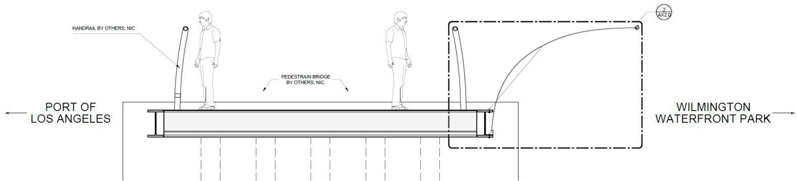
① SECTION, TYP. SCALE: 1"=2'-6"
